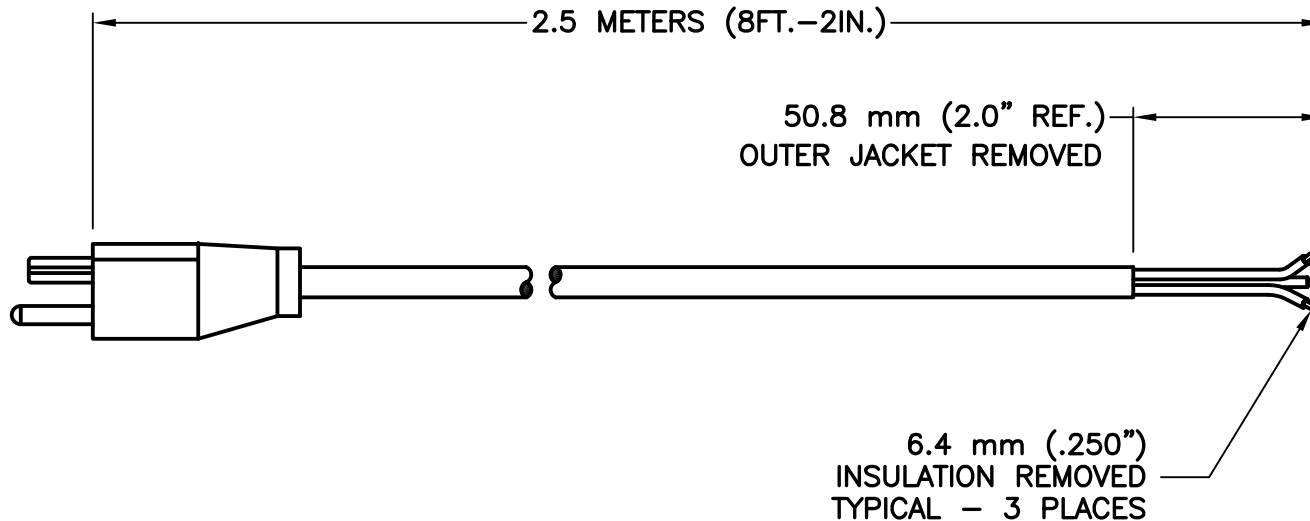
NEMA 5-20P
