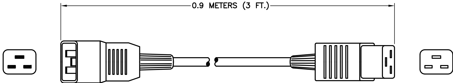
IEC 60320, C-20
