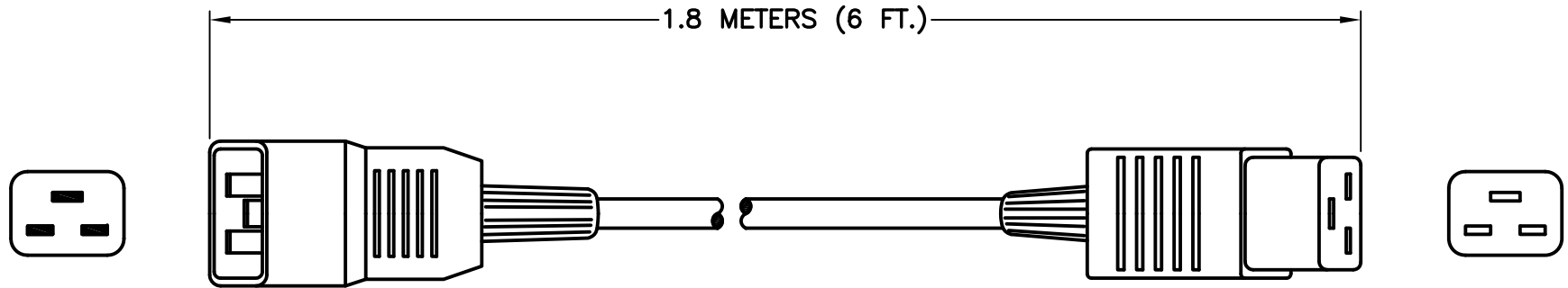
IEC 60320, C-20
