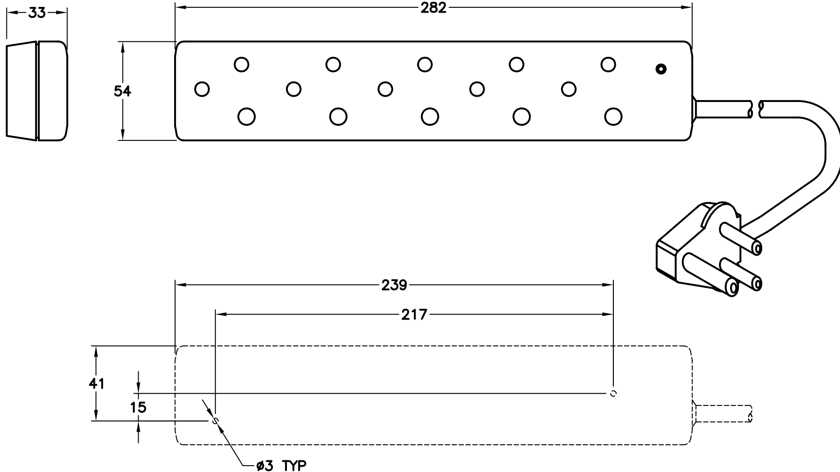
MOUNTING ARRANGEMENT
