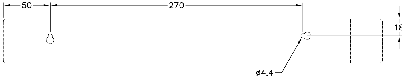
MOUNTING ARRANGEMENT
