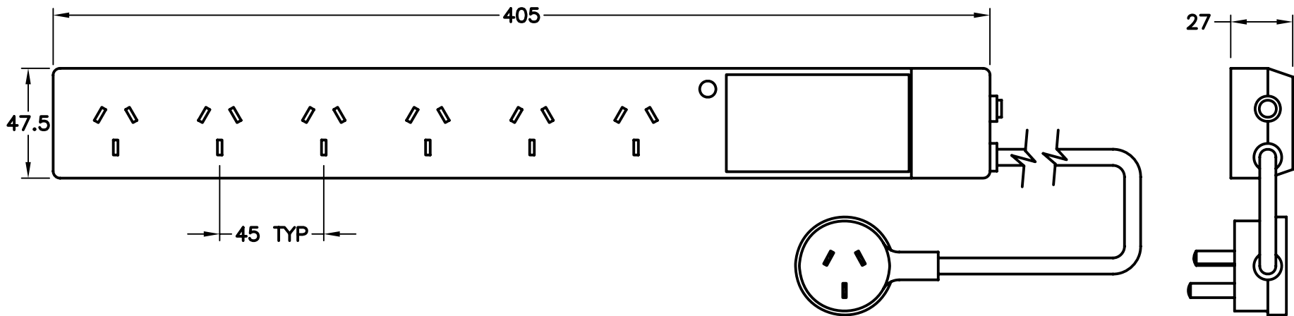
MOUNTING ARRANGEMENT
