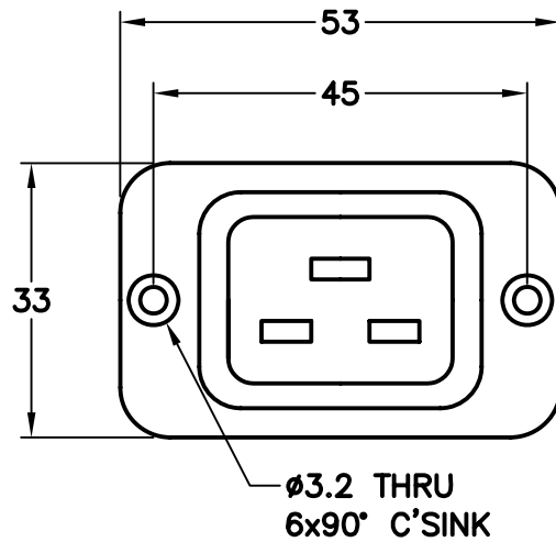
IEC 60320 C-19
