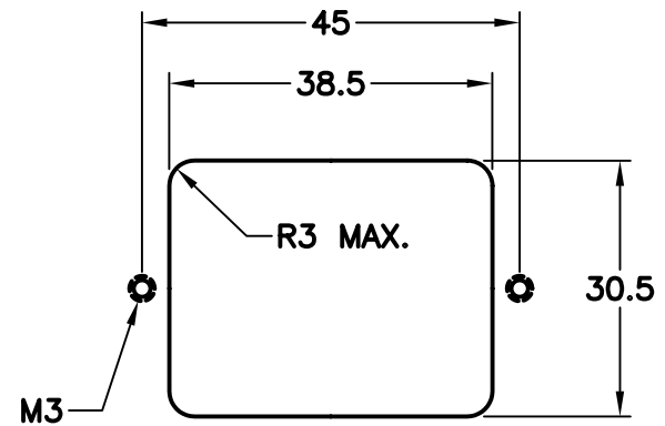
PANEL CUTOUT
