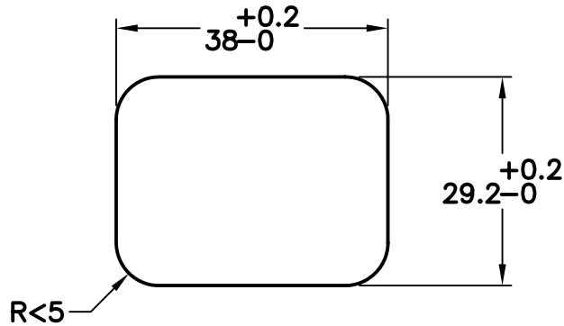
PANEL CUTOUT
