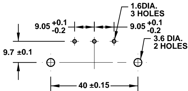
PIN SPACING
