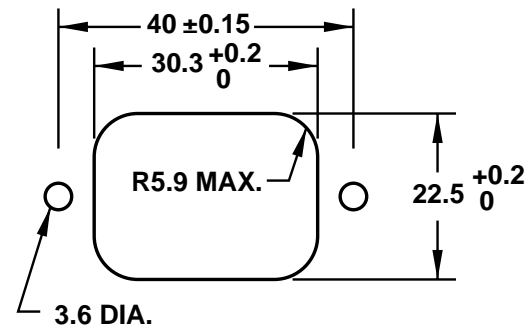
MOUNTINGHOLE
