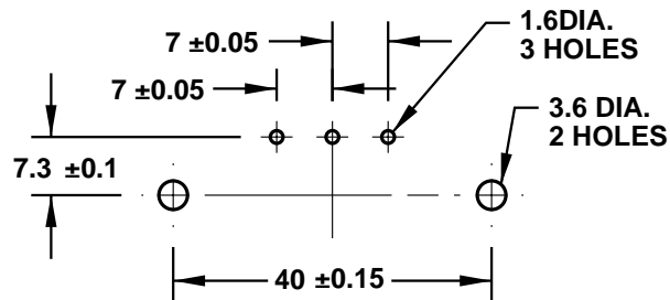
PIN SPACING
