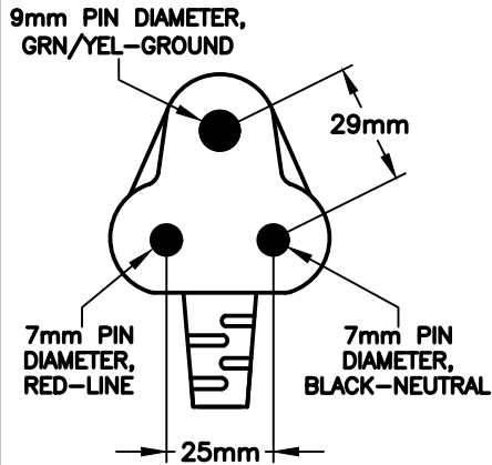
PLUG DIMENSIONS
