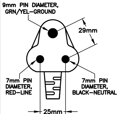
PLUG DIMENSIONS
