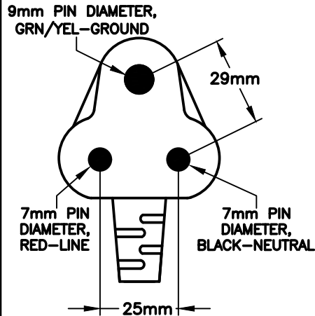
PLUG DIMENSIONS
