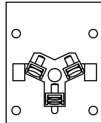
PANEL MOUNT DETAIL
