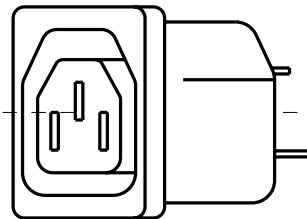
IEC 60320 (320) C-13 POWER OUTLET
