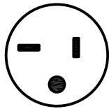
NEMA 6-20P HOSPITAL GRADE
