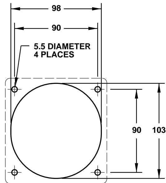
PANEL CUTOUT
